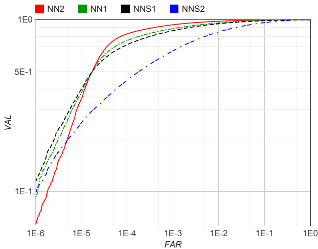
Figure 5. Network Architectures . This plot shows the complete ROC for the four different models on our personal photos test set from section 4.2. The sharp drop at 10^{-4} FAR can be explained by noise in the groundtruth labels. The models in order of performance are: NN2 : 224 \times 224 input Inception based model; NN1 : Zeiler&Fergus based network with 1 \times 1 convolutions; NNS1 : small Inception style model with only 220M FLOPS; NNS2 : tiny Inception model with only 20M FLOPS.
